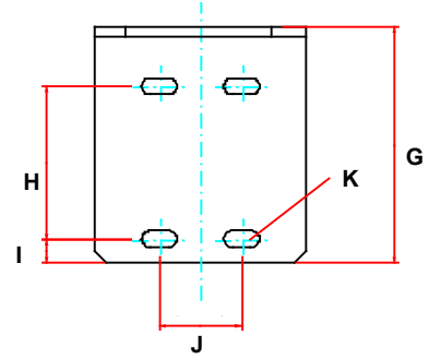
ABOVE VIEW
